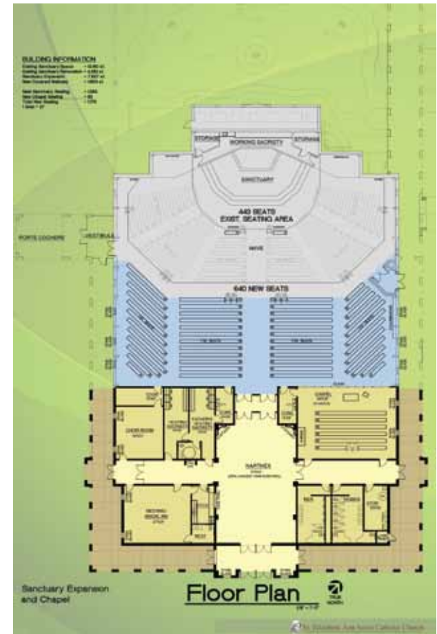
Floor Plan NTS
