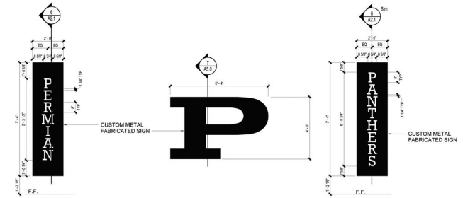
Signage Detail (NTS)
