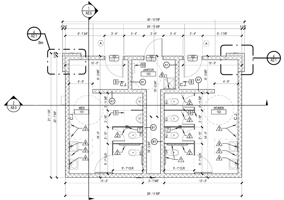
Floor Plan (NTS)
