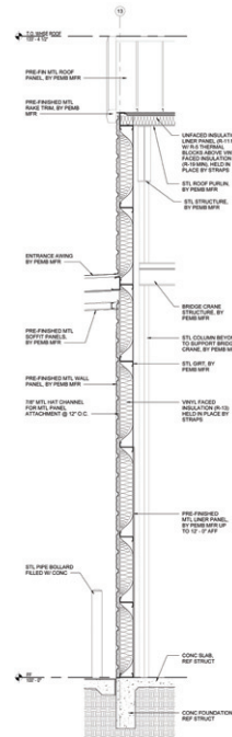
Wall Section (NTS)
