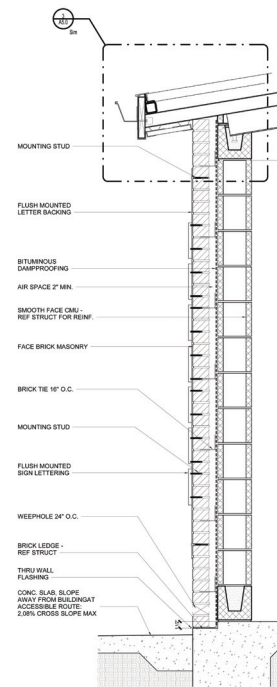
Wall Section (NTS)
