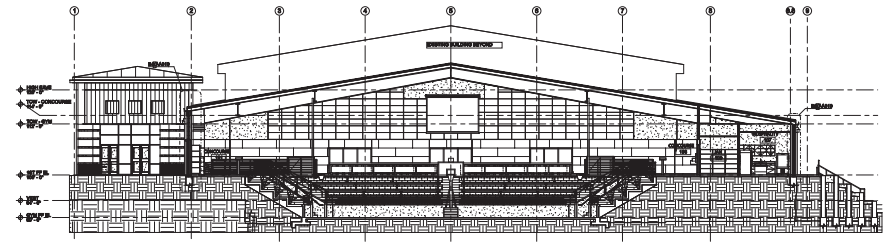
Transversal Building Section NTS
