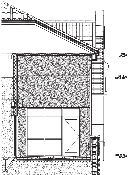
3rd Floor Wall Section NTS
