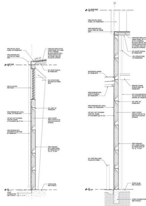
Wall Section (NTS)
